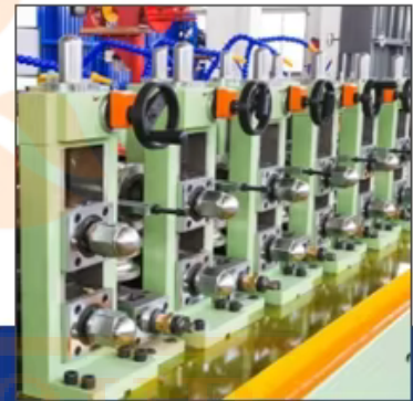
Forming and Sizing Machine
